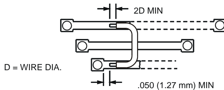
Figure 2 Connecting Two Conductors
