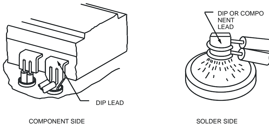
Figure 3 Wire Connections to DIP
