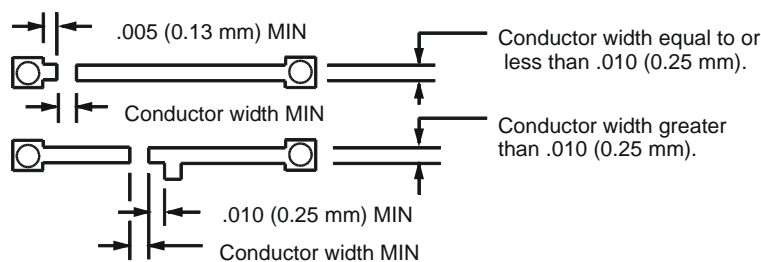
Figure 1 Conductor Modification
